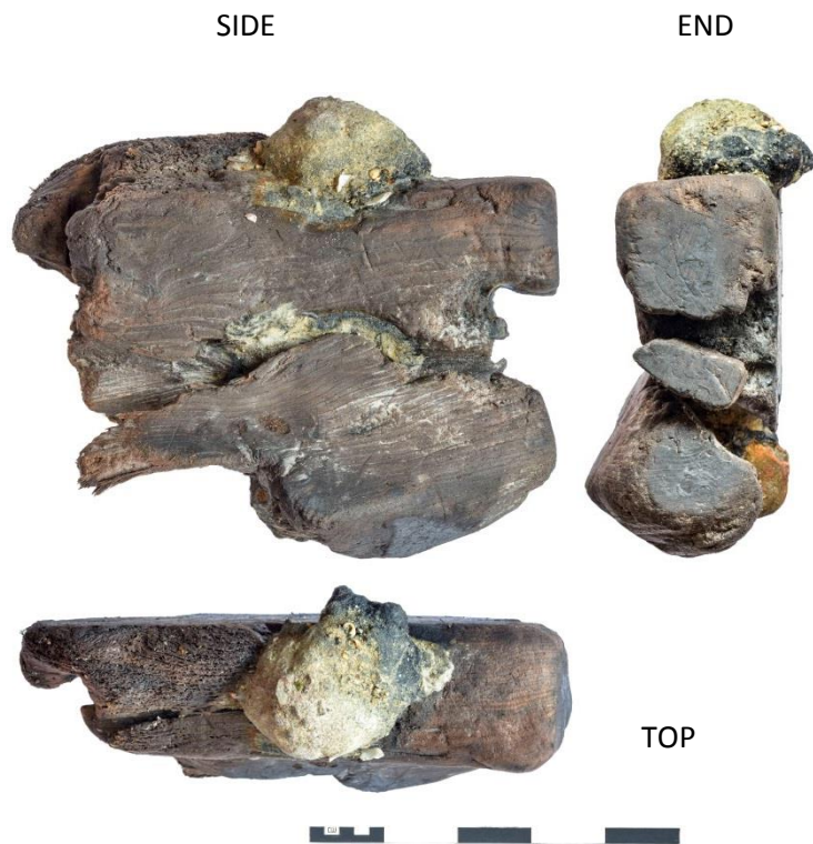
Fig 20 Three views of the timber gun carriage part 1240 with fragment 1265 in place. The side view shows how the timber has been broken and is only held together by the iron fastening. Scale = 0.25m
